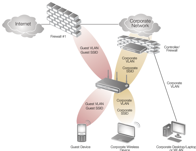
FIGURE 2: WLAN Implementation
